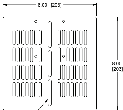
SLOTS FOR 1/4-20 OR M6
