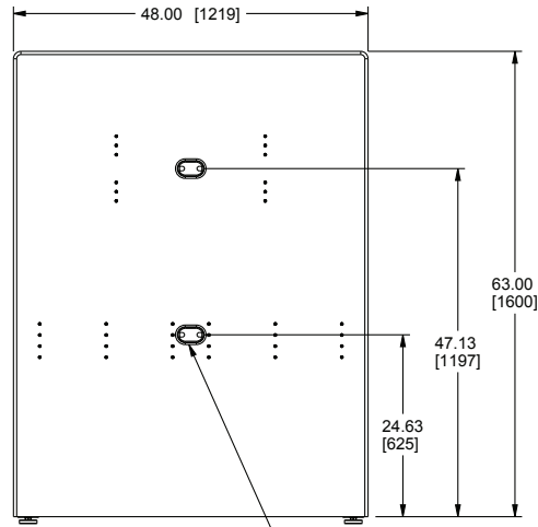
FRONT VIEW HUBTS-TOWERS-XXT
