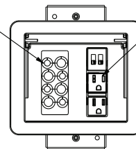
TB672AUBK TOP VIEW TOP COVER AND POWER CORD REMOVED FOR CLARITY
