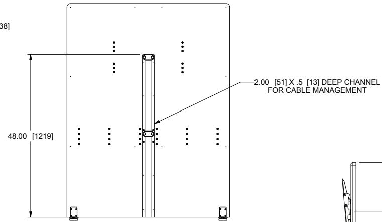
REAR VIEW HUBTS-TOWERS-XXT REAR COVER REMOVED FOR CLARITY
