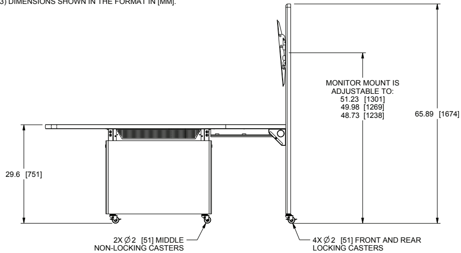
SIDE VIEW HUBTS-72ANGLE-H WITH INSTALLED HUBTS-TOWER5-XXT AND HUBTS-CASTER
