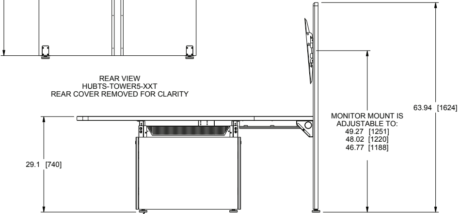
SIDE VIEW HUBTS-TOWERS-XXT
