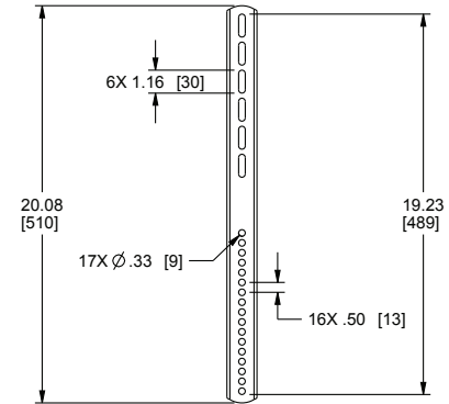
DISPLAY MOUNT BRACKET HOLE PATTERN
